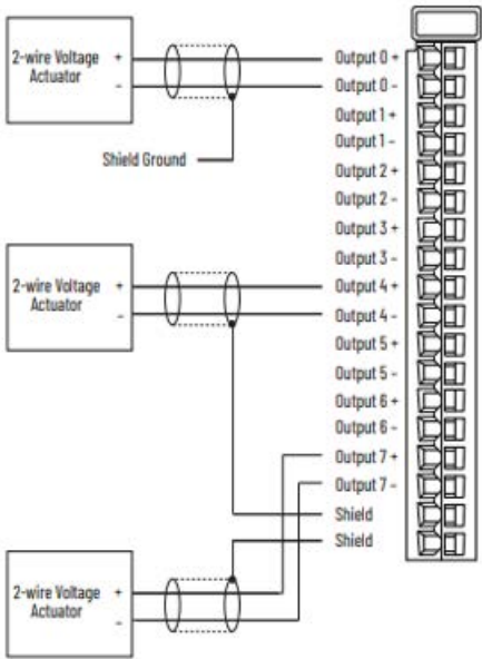
Voltage Mode Output Wiring - 5069-OF8
