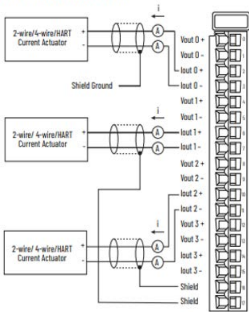
Current Devices Output Wiring - 5069-0F4IH
