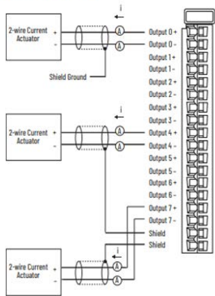
Current Mode Output Wiring - 5069-OF8
