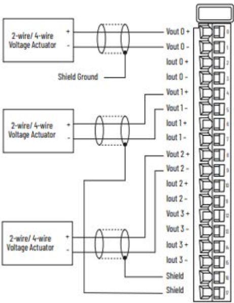
Voltage Devices Output Wiring - 5069-0F4IH
