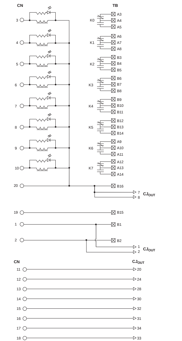
Relay Master (LED Indicating) 20-Pin Master With Eight (8) 24V DC Relays
